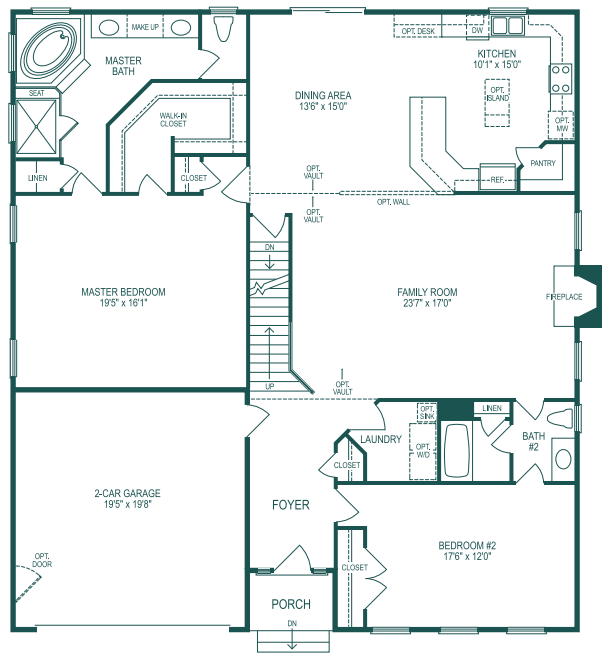
FIRST FLOOR PLAN EMERSON
