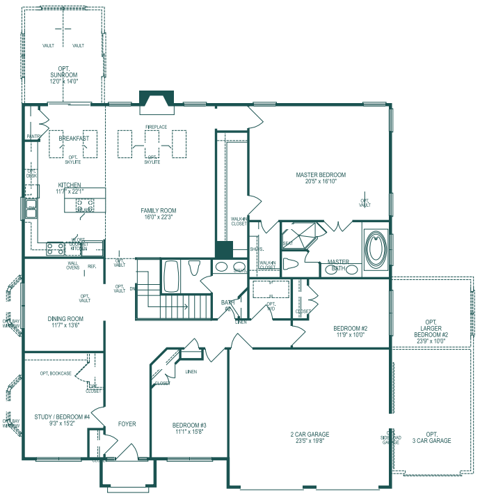
FIRST FLOOR PLAN OAKMONT EXTENDED
